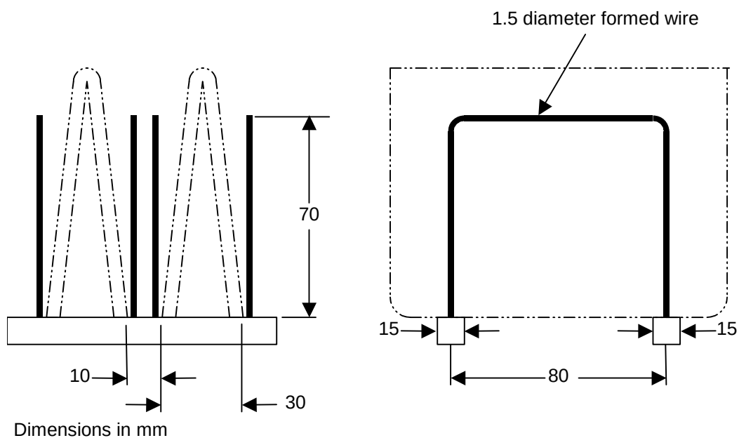
Figure 2 MRP rack
